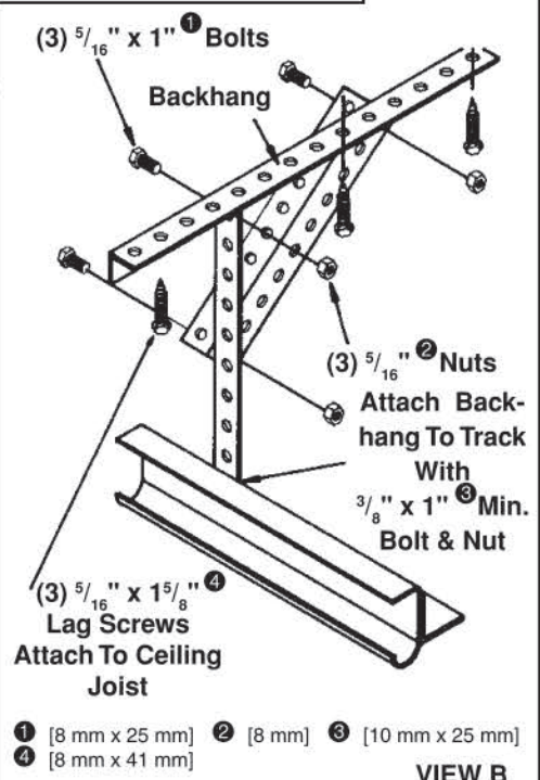
VIEW B
